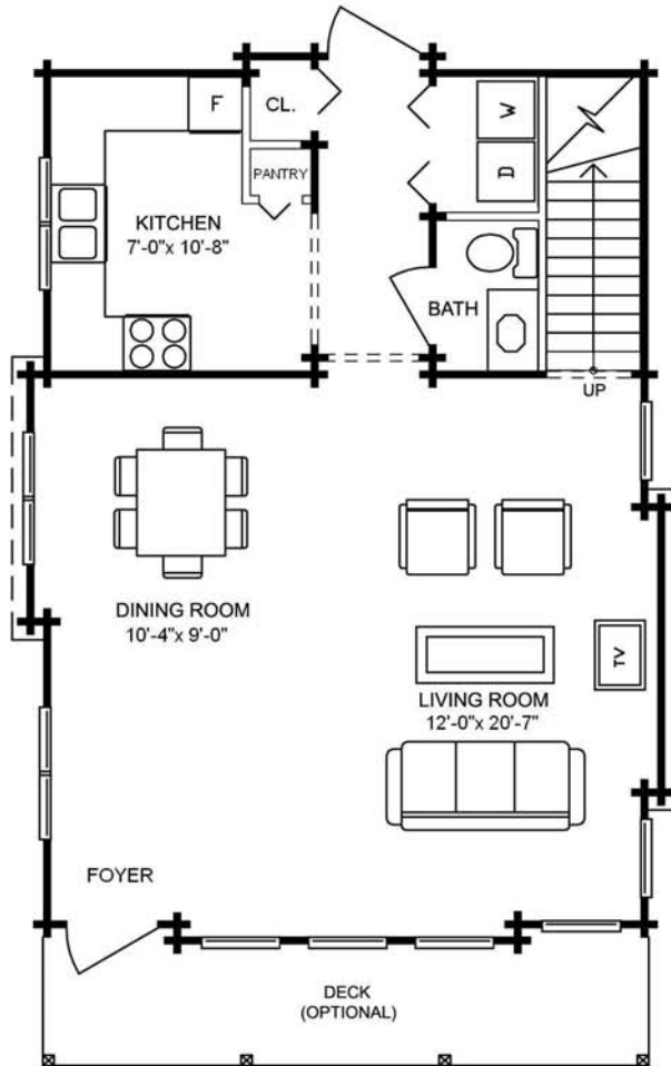
MAIN FLOOR PLAN 715 sq. ft. (66.43 sq. m.)
