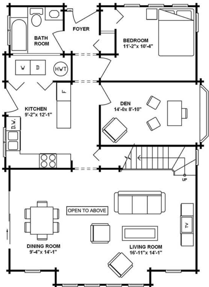
MAIN FLOOR PLAN 1053 sq ft (97.85 sq m)
