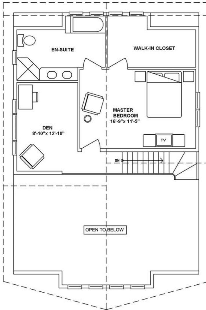
SECOND FLOOR PLAN 562 sq ft (52.22 sq m)
